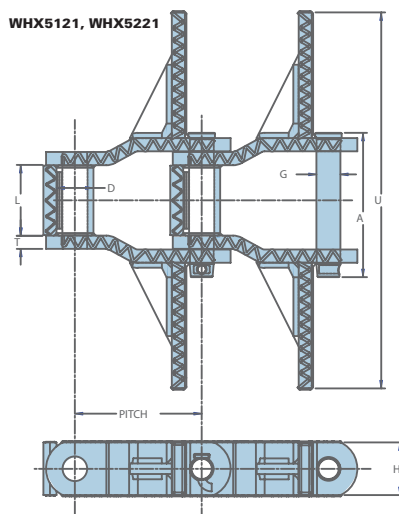
Chain runs closed end forward.
