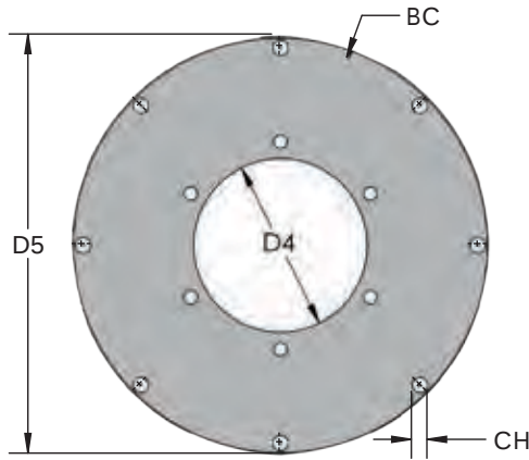
FIGURE 9 Flywheel
